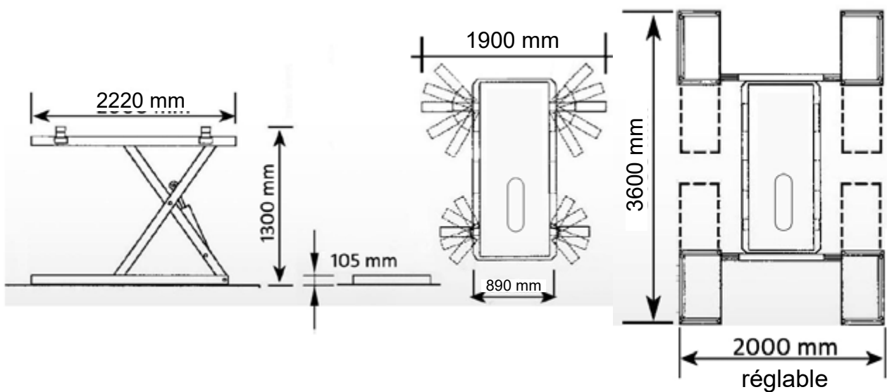
EH Electrohydraulique
